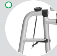
High level release For users who can't lean forward to release footplate catches.
